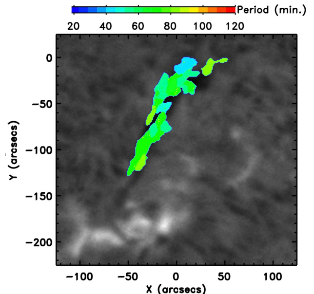
Fig. 12. Time periods of the filament oscillations over a GONG H\alpha image on January 1, 2014 using the technique developed by Luna et al. (2022a). The color code shows the periods in minutes.
