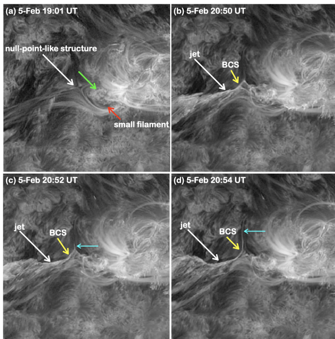
Fig. 3. Zoom image of the jet base in AIA 171 Å. The FOV for this figure is presented as the blue square in Fig. 1 (d). The null-point-like structure at the jet base is indicated with a white arrow (panel a). The jet is initiated under the arcade (green arrow) following a small filament eruption (red arrow). This small filament pushes the arcade toward the null-point like structure which leads to the jet flows towards the filament (white arrow in panel b-d) in the South-West. This flow is bidirectional, as we observe the second branch, which flows toward the North, is indicated with cyan arrows in panels (c-d). The null-point type structure collapses into the breakout current sheet (BCS). The latter is marked using yellow arrows in panels b-c-d. (See also the associated animation AIA171_feb.mov ).
