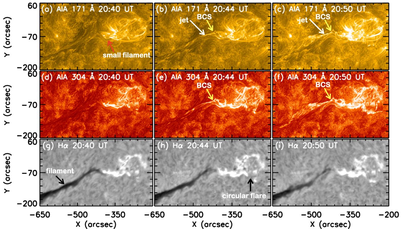
Fig. 4. Filament and jet evolution for event 1 on February 5, 2015 observed in AIA 171 Å (top row), in AIA 304 Å (middle row), in H \alpha (bottom row). The jet ejects from a dome-like structure with a small filament eruption shown in panel a. The jet flows towards the long filament through the BCS shown in panel b, c, e, and f and a zoomed view is presented in Fig. 3. The long filament is well observed in all these channels lying as a cool and dense structure (pointed in panel (g)). This jet is associated with a GOES B7.8 circular flare shown in panel h.
