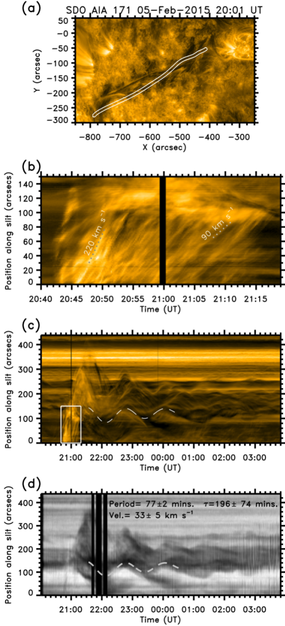
Fig. 5. Panel (a): Filament seen in absorption in AIA 171 Å on February 5, 2015, with the artificial slit used to construct the time-distance diagrams (panels b-d) shown as a white contour. (Panel b) time-distance diagram for the AIA171 image along the topmost 150'' of the slit; panel (b) in Fig. 3, taken at time 20:50 UT. Panels c and d contain the time-distance diagrams for the brightness in along the curved slit, clearly showing the oscillatory patterns analyzed in the paper. The white tracks in panels c and d show one of the fits obtained for the oscillation which has period 77 min, velocity amplitude 33 \text{ km s}^{-1} and damping time \tau = 196 \text{ min} . The black vertical stripes in panels (b), (c) and (d) are data gaps.
