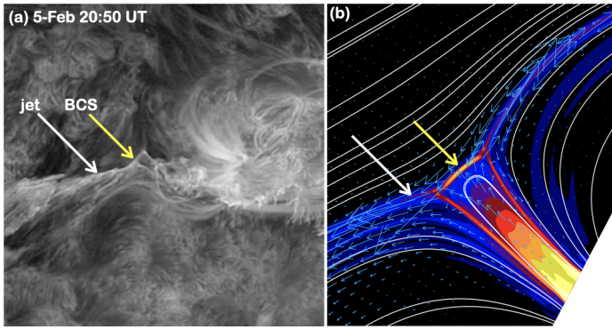
Fig. 7. Similarity between the observation of event 1 on February 5, 2015 and the numerical model of Luna & Moreno-Insertis (2021). The left panel is identical to panel b of Fig. 3; the right panel shows the electric current distribution of the model of Luna & Moreno-Insertis (2021) (adapted from their Fig. 4c). The flat breakout current sheet is marked in both panels by a yellow arrow.
