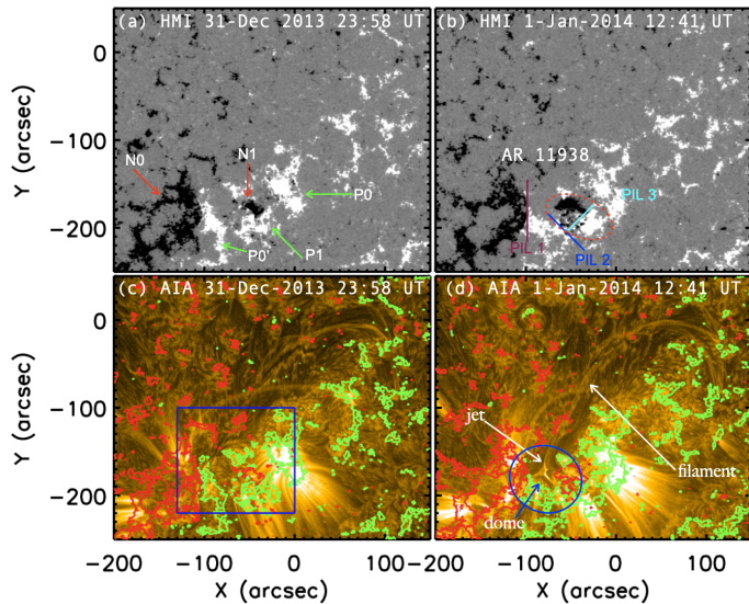
Fig. 9. Evolution of magnetic field (top row) and filament channel in AIA 171 Å (bottom row) for event 2. The AR 11938 consists a big positive polarity patch (P0', P0, and P1) surrounded with negative polarities (NO, N1). The different PILs (1, 2, 3) are shown in panel (b). The filament appears as dark areas (panel (c-d)) and the bright thin loops are possibly arcades or magnetic field lines of the filament structure. The jet flowing towards the filament channel near the PIL2 is shown with arrow in panel (d). The dome and null-point-like structure is enclosed by a blue circle. The green and red contours in the bottom row are the HMI magnetic field contours of strength \pm 50 Gauss respectively. All images are aligned together at January 1, 2014 at 15:56 UT. Blue rectangular box is the FOV for Fig. 13.
