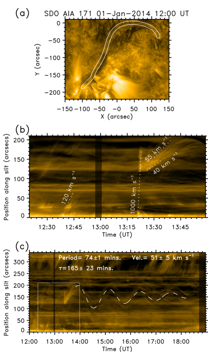
Fig. 11. Tracing of the oscillations in the filament for the first event on January 1, 2014 observed with AIA 171 Å. Figure showing the filament seen in absorption in AIA 171 Å. The artificial slit is shown as a white contour shown in panel (a) to construct the time-distance diagram shown in panels (b) and (c).
