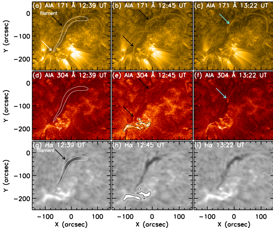
Fig. 10. Filament and jet evolution on January 1, 2014 (event 2) in AIA 171 Å (top row), AIA 304 Å (middle row), and H \alpha (bottom row). The null-point-like structure is shown with a white arrow in panel (a) at the top of the dome-like structure. The jet propagation from this null-point towards the filament channel is shown with black arrows (panel (b) and (e)). The cyan arrows in panel (c) and (f) show the later brightening associated with the jet, which reinforces the oscillations. The filament is very well observed in H \alpha as a dark long structure shown with black arrow in panel (g). The contours of the filament observed in H \alpha are over-plotted in AIA 171 and 304 Å channels (panels a,b,d). The black contours in panel (e) and (h) are for the brightening at the jet base observed in H \alpha overplotted in AIA 304 Å.
