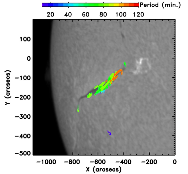
Fig. 6. Time periods of the filament oscillations over a GONG H \alpha image on February 5, 2015 using the technique developed by Luna et al. (2022a). The color code shows the periods in minutes.
